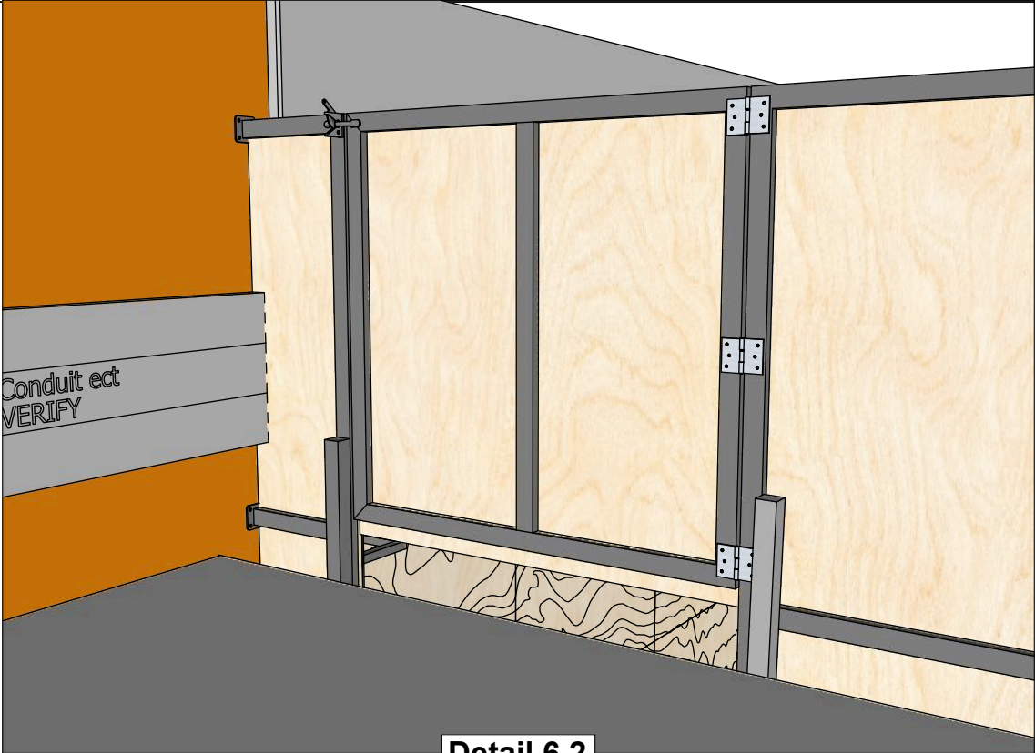
Detail 6.2
