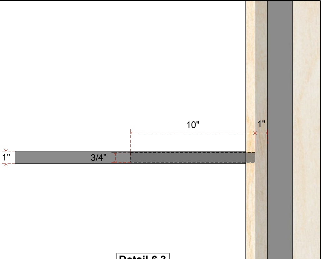
Detail 6.3
